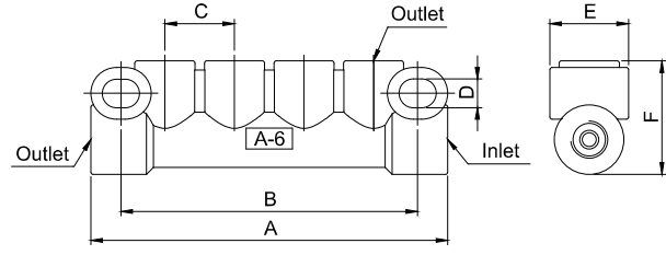
Dimensional Drawing of A-6-6-4
