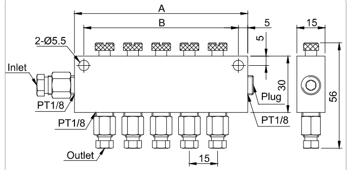
Dimensional Drawing of B-5-6-4
